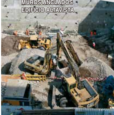
SOIL NAIL
