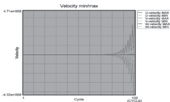
Figure 12. Velocity Min/Max plot of poorly meshed pit.
