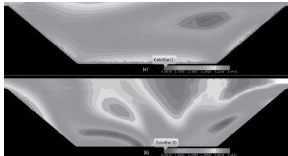
Figure 14. Magnitude of velocity contour plot of (a) No Prism Mesh and (b) Pit Boundary prism mesh.
