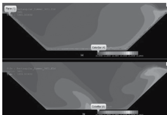
Figure 15. Temperature contour plot of (a) No Prism Mesh and (b) Pit Boundary prism mesh.
