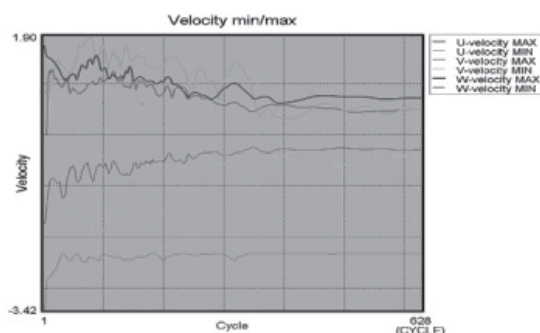
Figure 13. Velocity Min/Max plot of good quality mesh.
