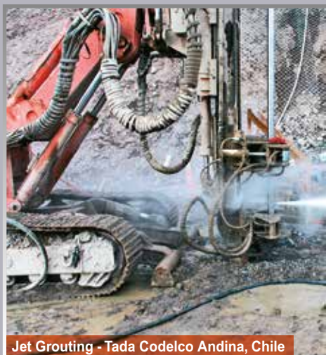
Jet Grouting - Tada Codelco Andina, Chile
